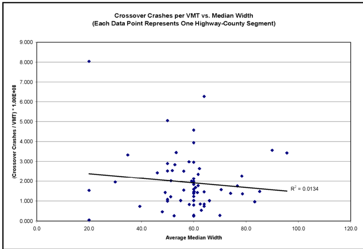
FIGURE 3 Crossover median crash rates vs. average median width.
